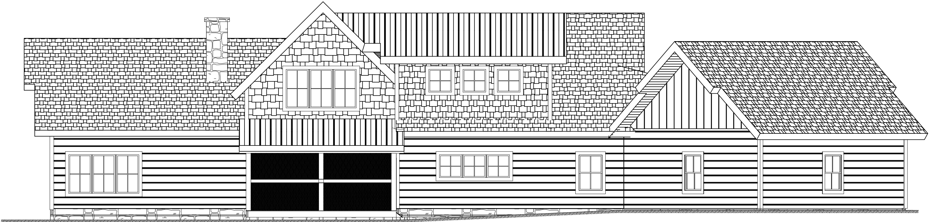
REAR ELEVATION NOTE: GRADE CONDITIONS TO BE VERIFIED ON SITE
